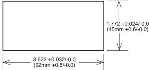
PANEL CUTOUT
