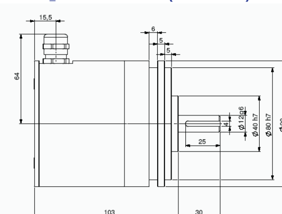
DHM9_12 connection GBR (terminal box)
