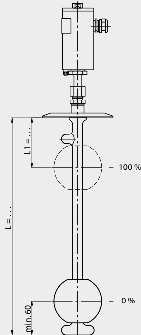
Tri - clamp with box Type AVVTC ...
