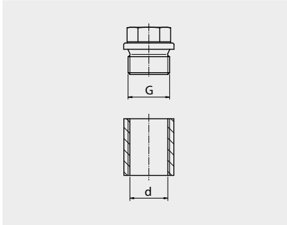
Thread R ..."
