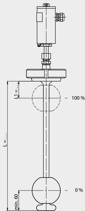
Tube connection with box Type AVVBKNW ...
