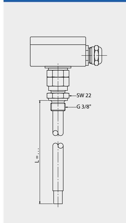
Thread with terminal box type ALVR3/8 ...
