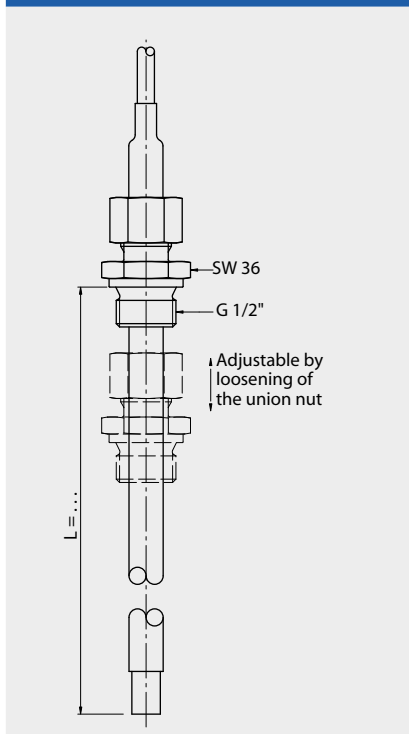
Thread with cable type EVR1/4 - ... adjustable
