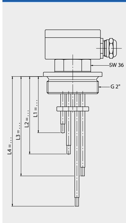
Thread with terminal box type ALVR2 ...
